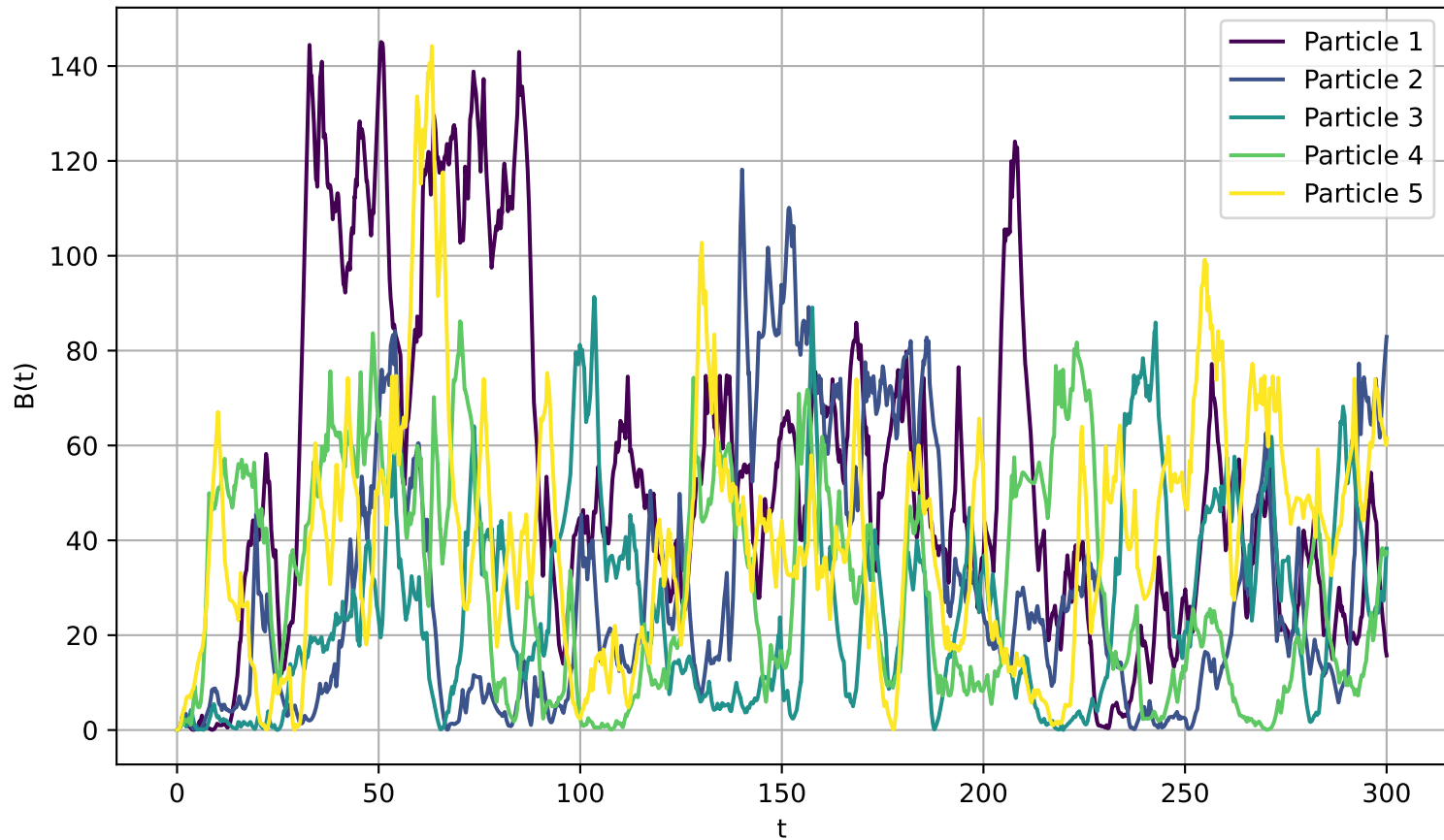
Brownian Motion without Noise
